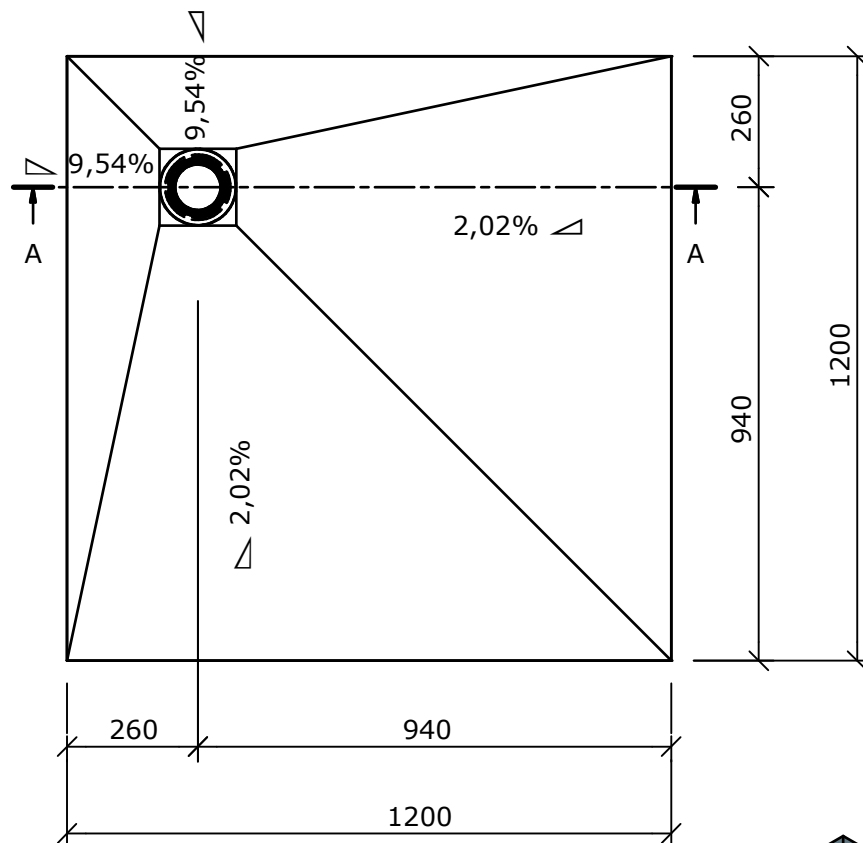
top view ( 1 : 15 )
